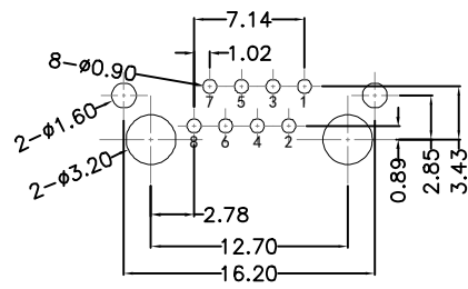
RECOMMENDED PCB LAYOUT VIEWED FROM COMPONENT SIDE
