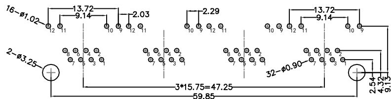
RECOMMENDED PCB LAYOUT VIEWED FROM COMPONENT SIDE
